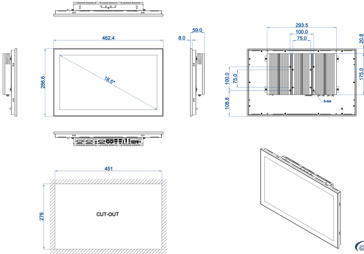
DIMENSIONAL DRAWING:TPC-DCT185D
