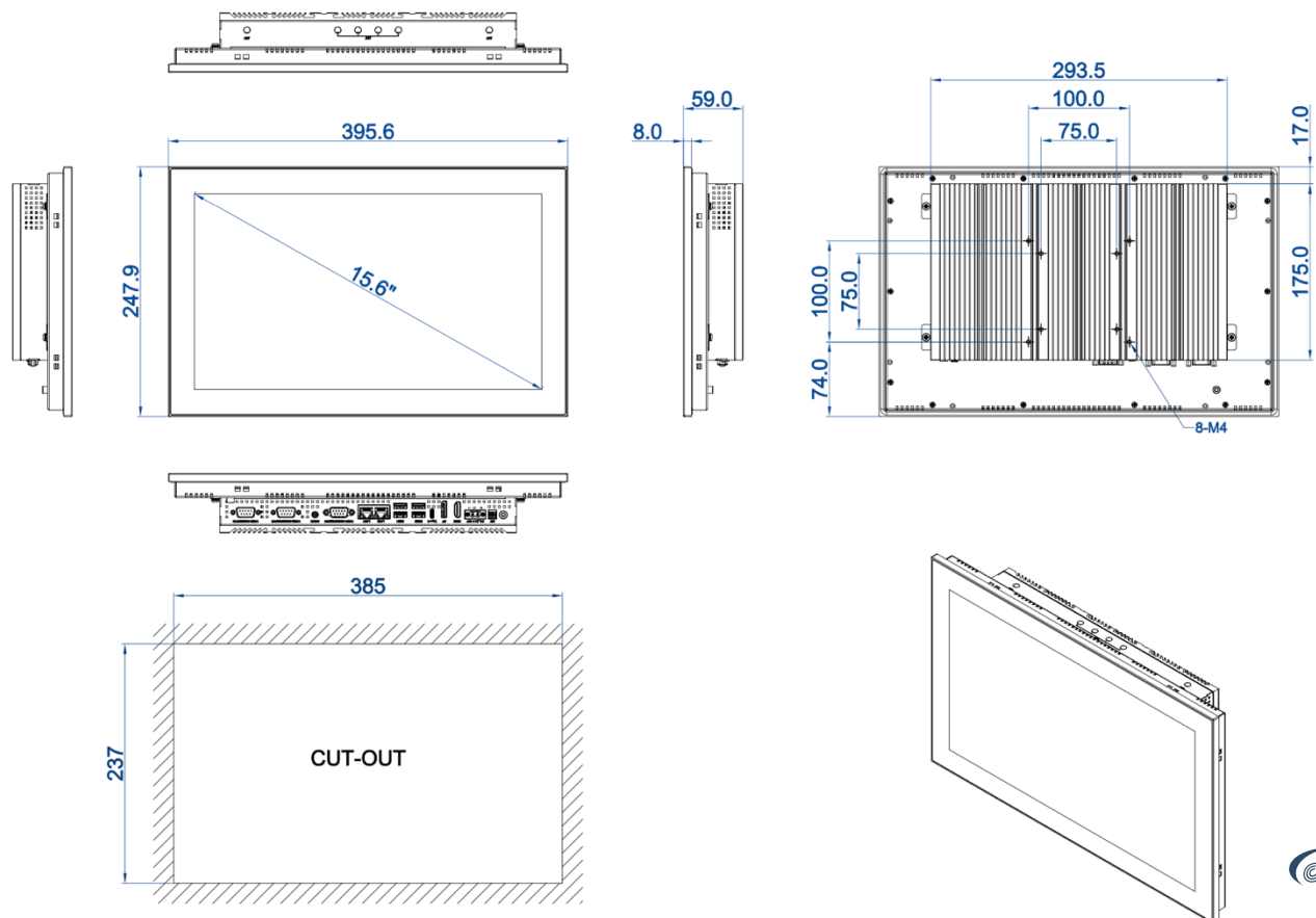
DIMENSIONAL DRAWING:TPC-DCT156D
