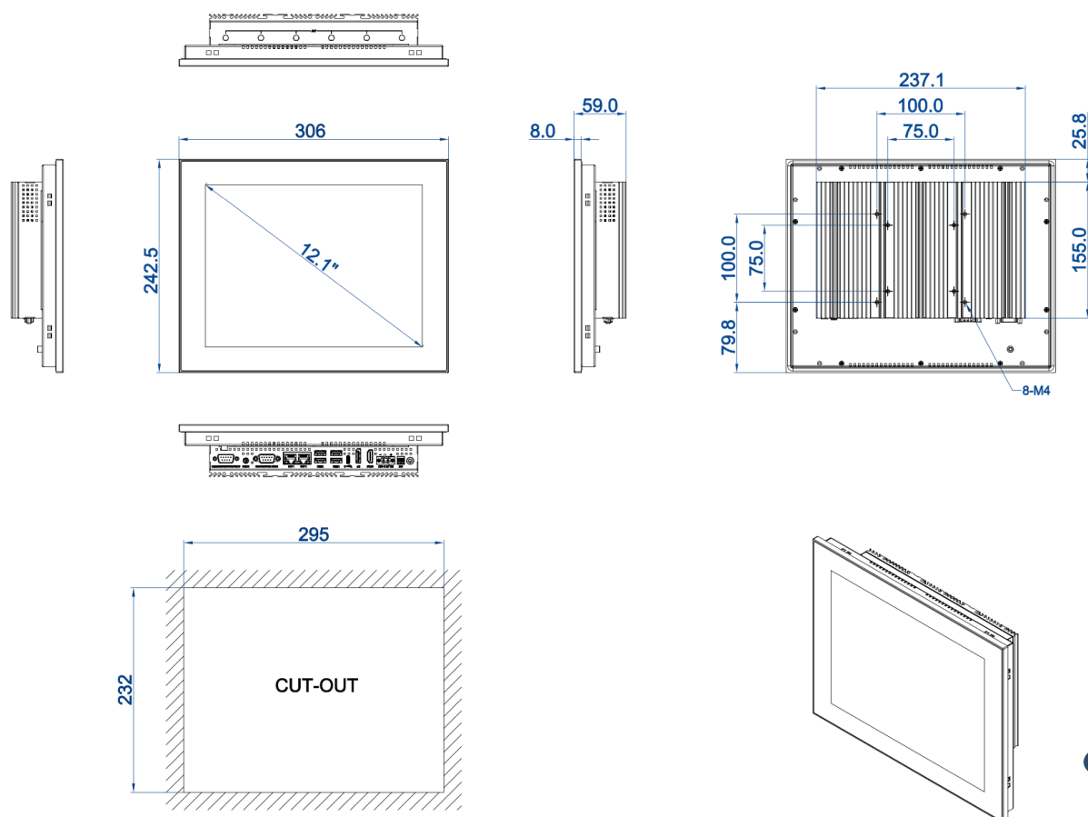
DIMENSIONAL DRAWING:TPC-DCT121D
