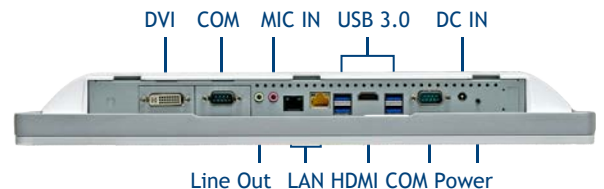
Line Out LAN HDMI COM Power
